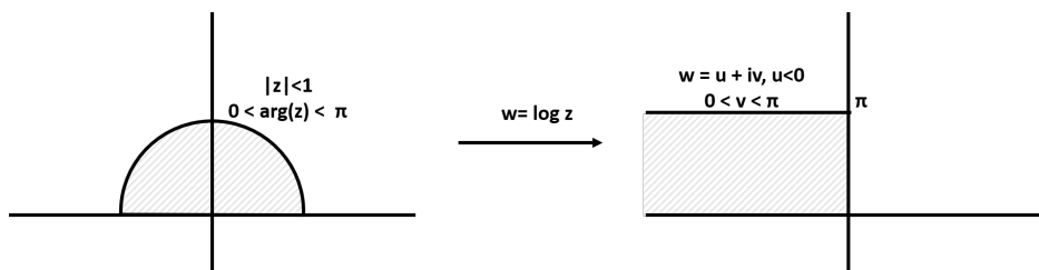
Figure 22.4: The logarithm mapping a semi-circular region into a half infinite strip
